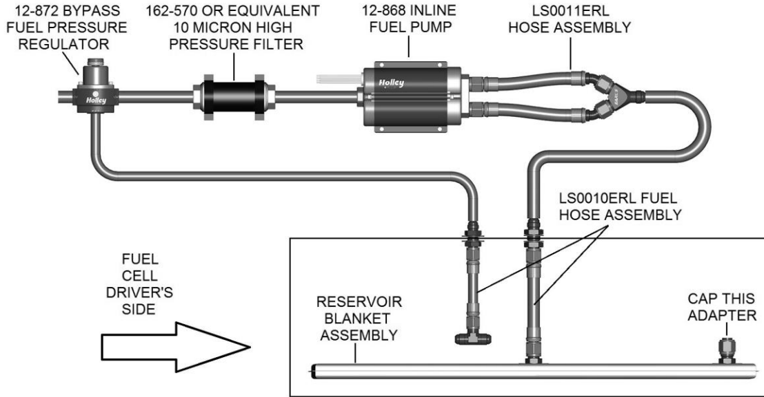
Figure 20 – 12-868 Fuel Pump
