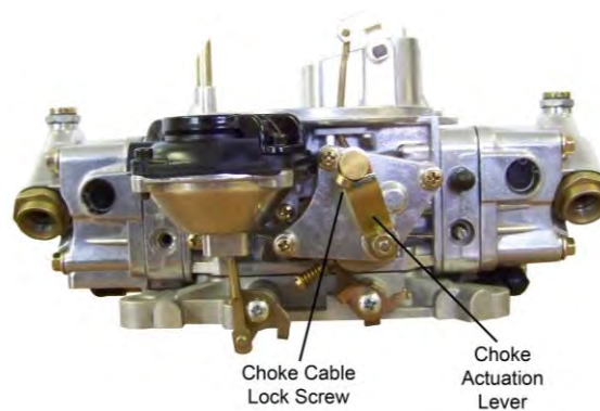
Manual choke parts (0-85770 shown)
